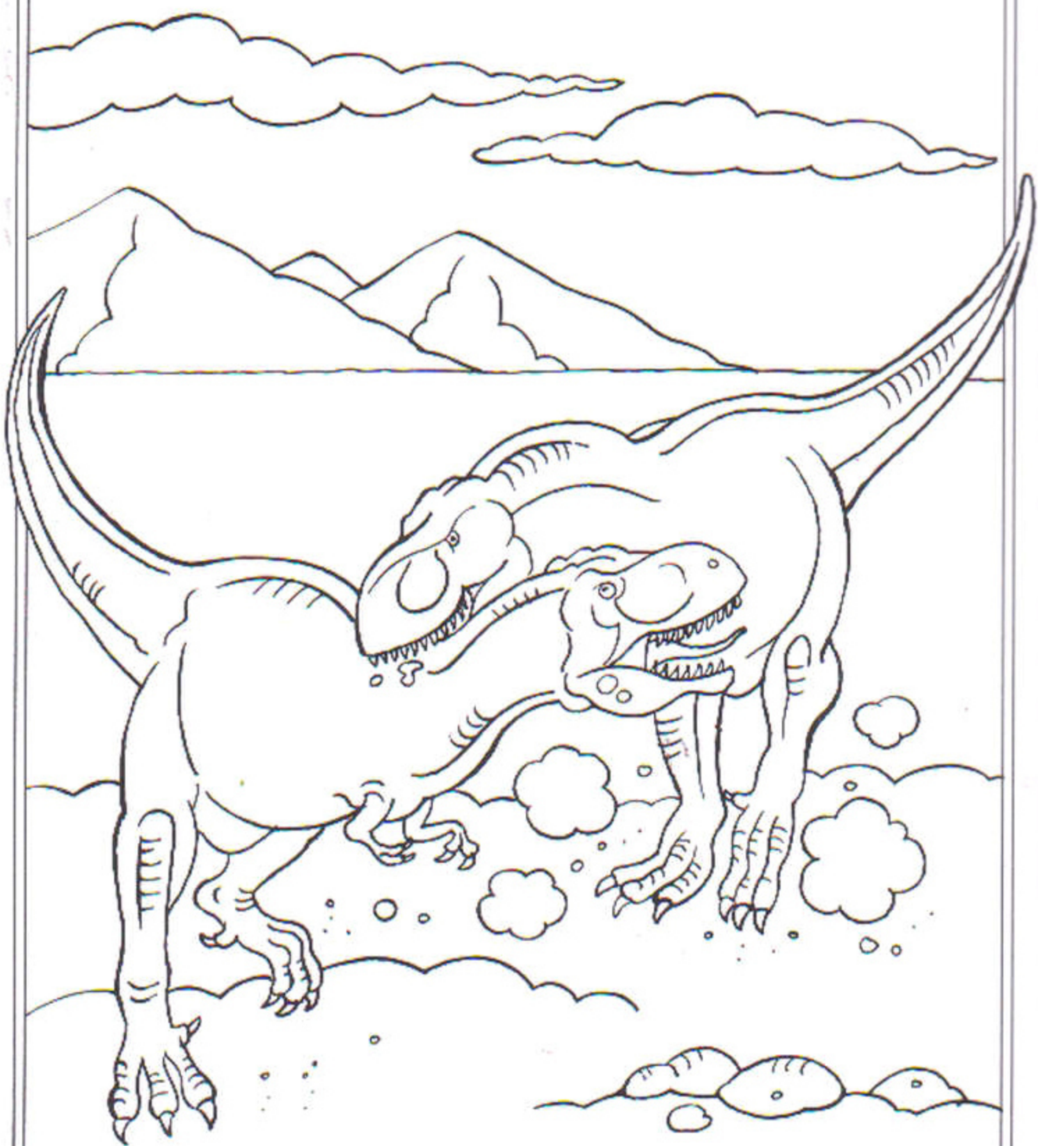
Tyrannosaurus rex
